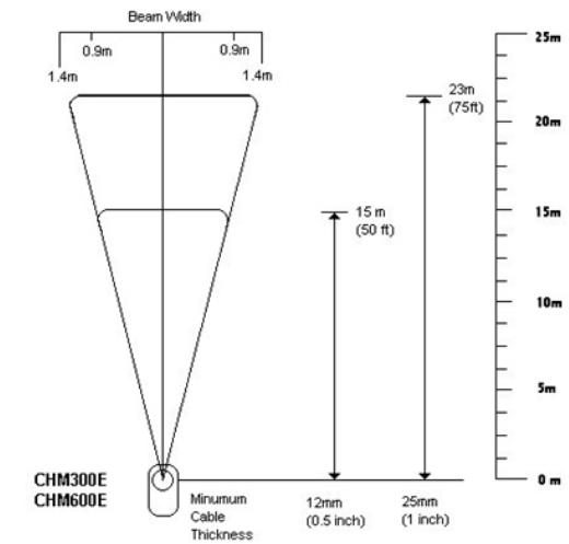
CHM Measurement versus Cable Thickness
