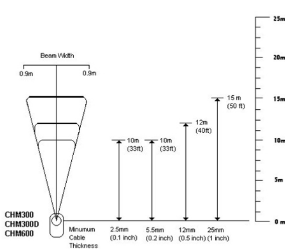
CHM Measurement versus Cable Thickness
